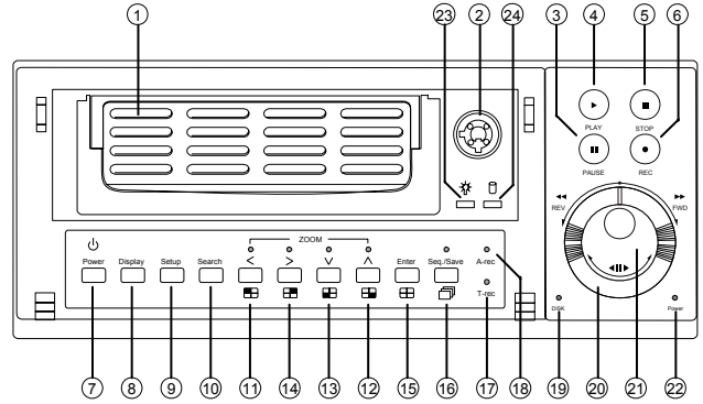
DVR-3024M (FOR REMOVABLE HDD MODEL)
